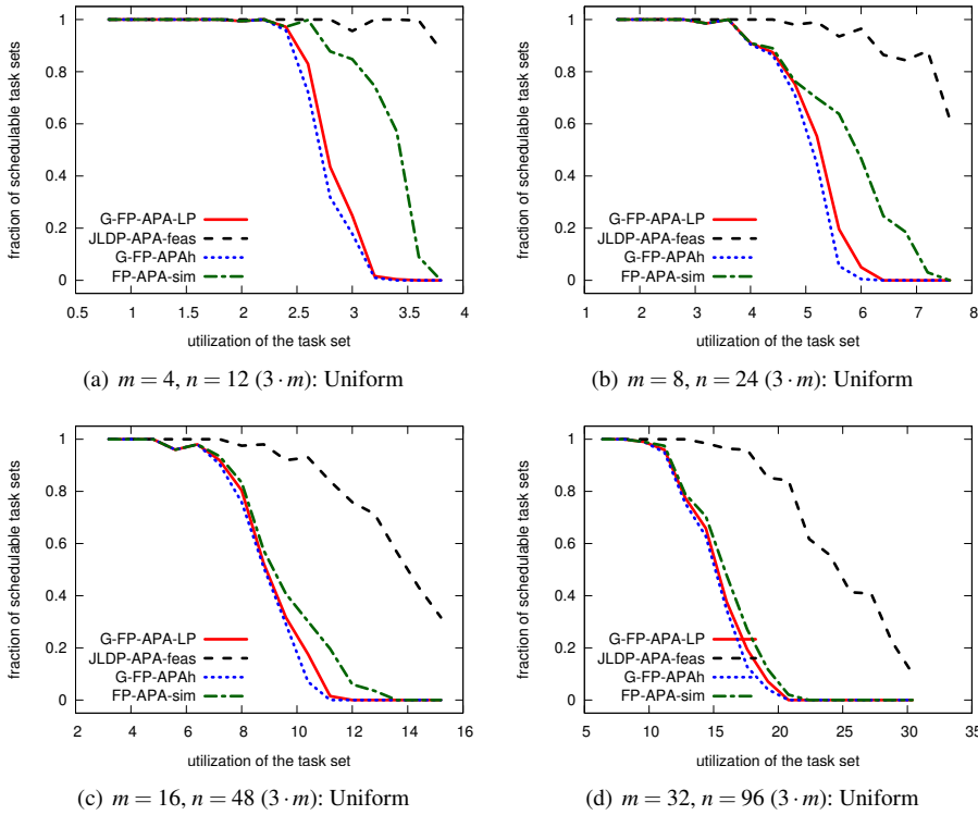
Fig. 6 The comparison of the LP-based Analysis (G-FP-APA-LP) with the APA Feasibility Test (JLDP-APA-feas), the heuristic-based reduction (G-FP-APAh) and the APA simulation (FP-APA-sim), for tasksets generated using uniform distribution with a fixed tasks-per-processor ratio of 3.
