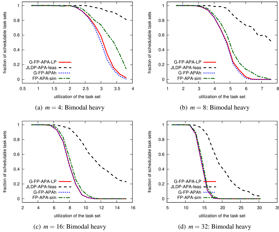
Fig. 5 The comparison of the LP-based Analysis (G-FP-APA-LP) with the APA Feasibility Test (JLDP-APA-feas), the heuristic-based reduction (G-FP-APAh) and the APA simulation (FP-APA-sim), for tasksets generated using the bimodal heavy distribution.
